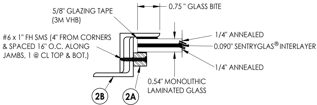
G3 GLAZING DETAIL Operable Door/Sidelite
