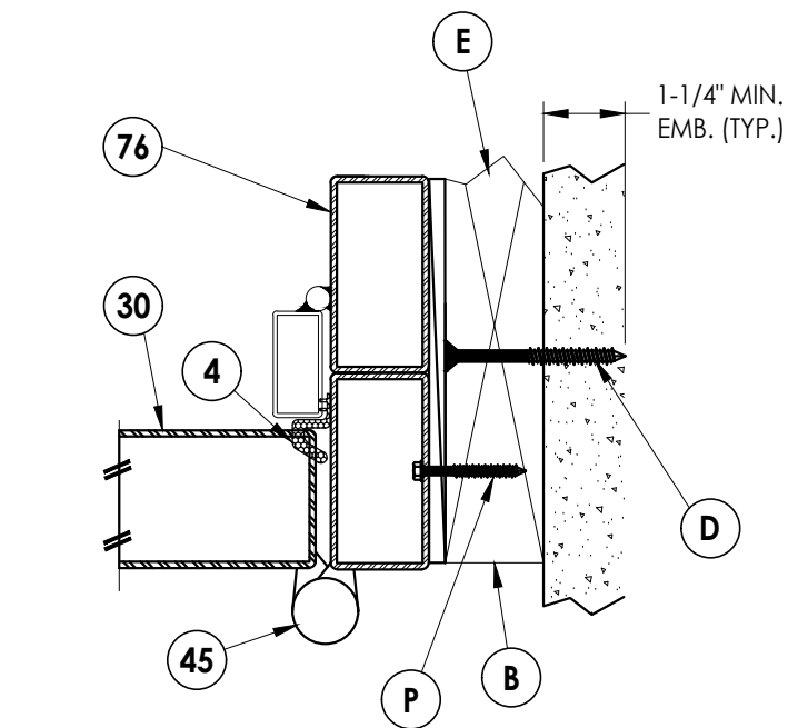
2 HORIZONTAL CROSS SECTION 4 Shown w/ Optional Through the Frame Anchoring
